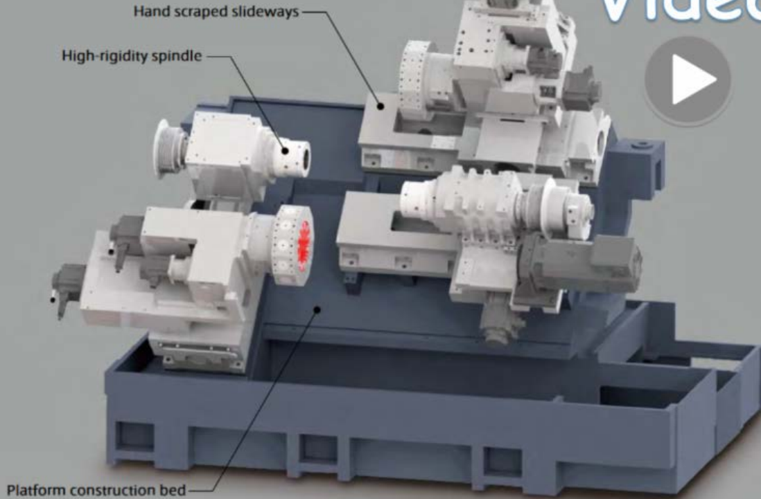
Basic construction of the BNE-51MSY
